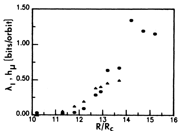
FIG. 2. The largest Lyapunov exponent \lambda_1 (dots) obtained from five-dimensional phase portraits and the metric entropy h_\mu (triangles) as a function of R . The units are bits per orbit (i.e., bits per intersection with a Poincaré section). For calculations of \lambda_1 and h_\mu the data were low-pass filtered with a cutoff at approximately 3 times the higher fundamental frequency.
