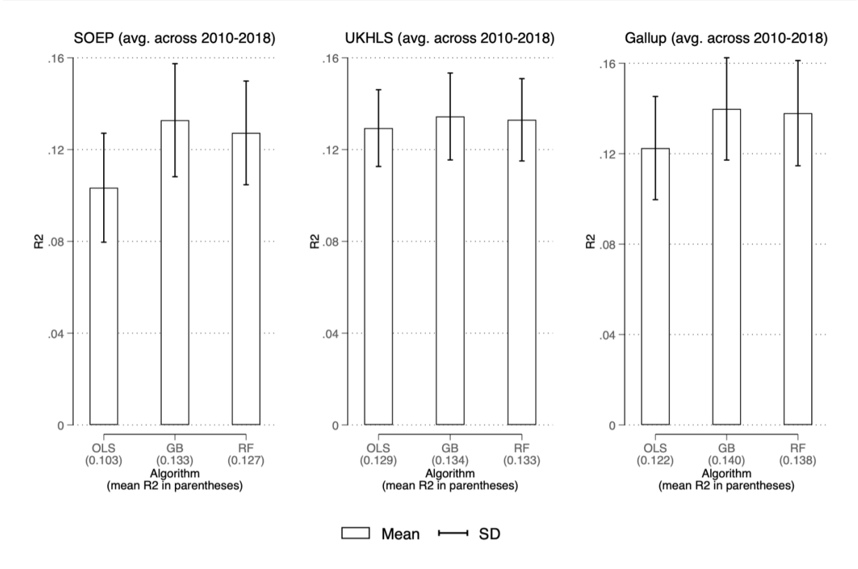
Figure 1: R-squared figures from OLS, GB and RF using the restricted set of variables. The R-squareds are computed using the unseen testing data.
