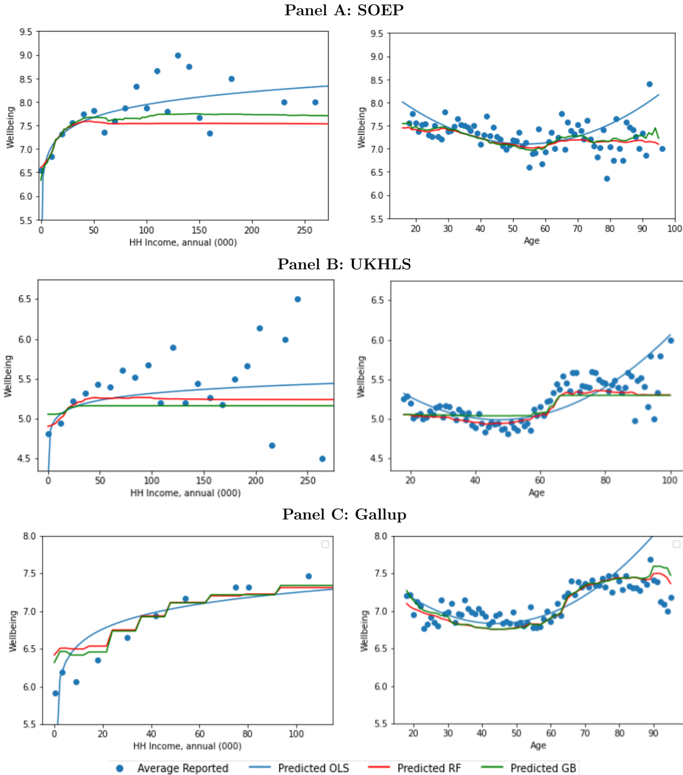
Figure 4: The mean effects of age and household income on wellbeing, restricted set of variables.
